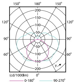
LED Lamps, CorePro R7S 118mm 14-100W /830 D
